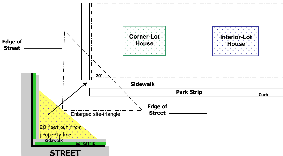
Site Plan
